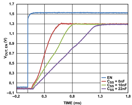
Figure 25. Fixed V_{OUT} Ramp-Up with External Soft Start Capacitor ( V_{OUT, EN} ) vs. Time
