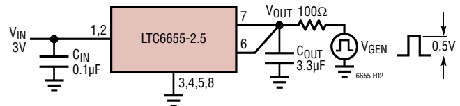
Figure 2. Transient Load Test Circuit
