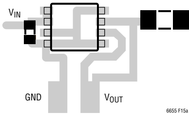
Figure 15a. Sample LTC6655 PCB Layout
