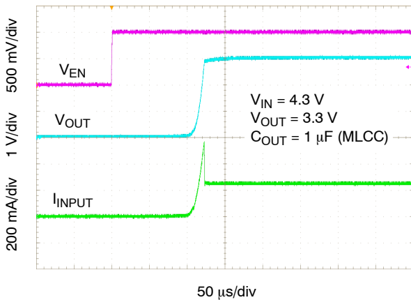
Figure 34. Enable Turn-on Response – C_{OUT} = 1 \mu F, I_{OUT} = 250 mA – “A” Option
