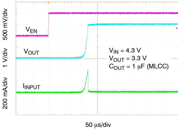
Figure 32. Enable Turn-on Response – C_{OUT} = 1 \mu F, I_{OUT} = 10 mA – “A” Option
