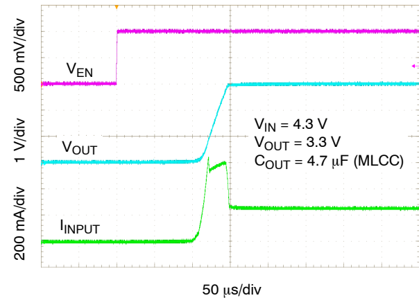
Figure 35. Enable Turn-on Response – C_{OUT} = 4.7 \mu F, I_{OUT} = 250 mA – “A” Option
