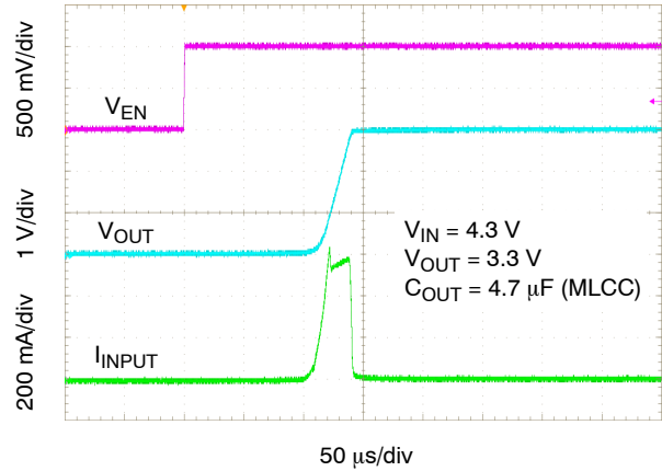
Figure 33. Enable Turn-on Response – C_{OUT} = 4.7 \mu F, I_{OUT} = 10 mA – “A” Option
