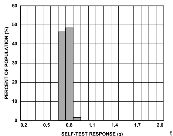
Figure 19. X-Axis Self-Test Response at 25°C, V_S = 2.5\text{ V}
