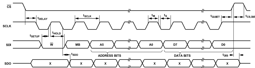
Figure 27. SPI 4-Wire Write
