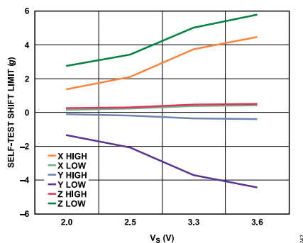
Figure 33. Self-Test Output Change Limits vs. Supply Voltage
