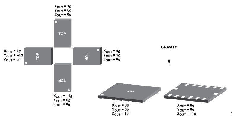
Figure 48. Output Response vs. Orientation to Gravity
