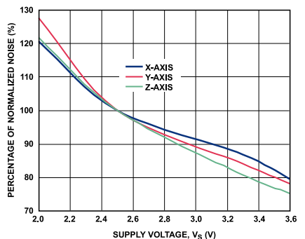
Figure 43. Normalized Noise vs. Supply Voltage, V_S
