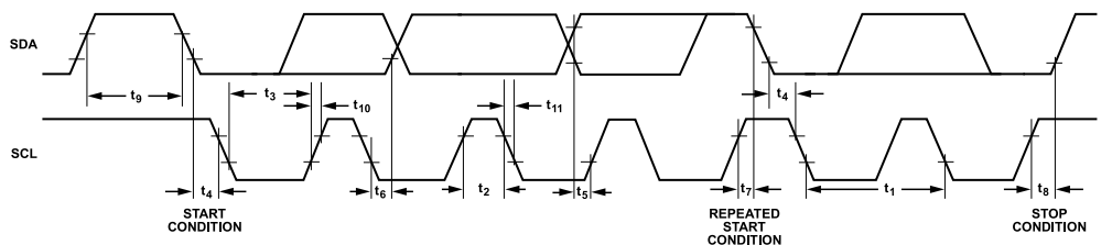
Figure 32. I 2 C Timing Diagram
