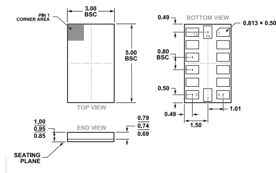
Figure 50. 14-Terminal Land Grid Array [LGA] (CC-14-1) Dimensions shown in millimeters
