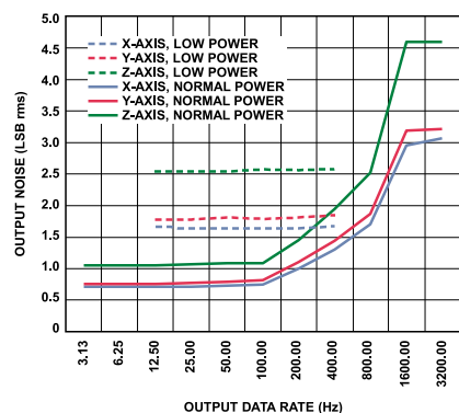
Figure 41. Noise vs. Output Data Rate for Normal and Low Power Modes, Full-Resolution (256 LSB/g)
