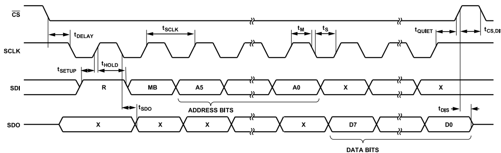
Figure 28. SPI 4-Wire Read
