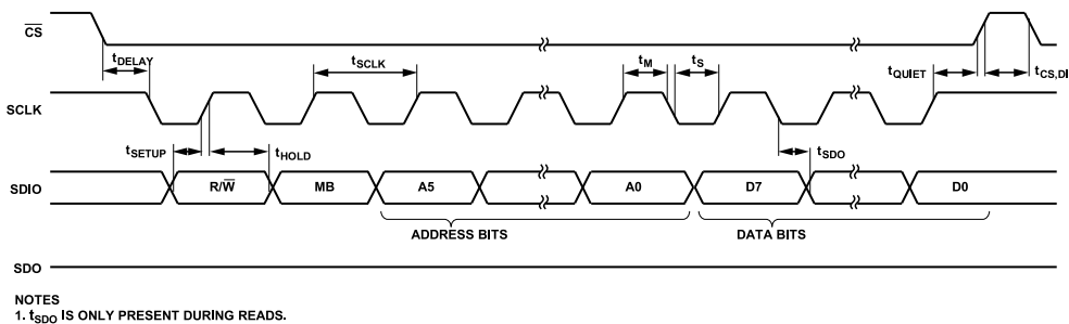
Figure 29. SPI 3-Wire Read/Write
