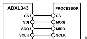
Figure 25. 4-Wire SPI Connection Diagram
