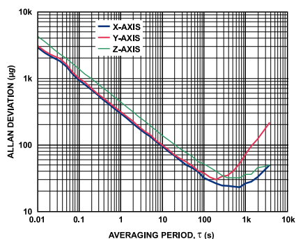
Figure 42. Root Allan Deviation
