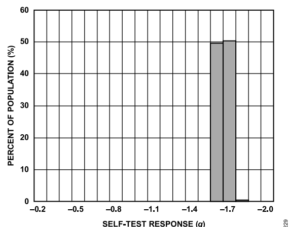
Figure 20. Y-Axis Self-Test Response at 25°C, V_S = 2.5\text{ V}
