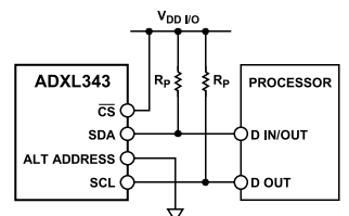
Figure 30. I 2 C Connection Diagram (Address 0x53)
