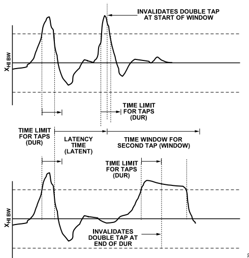
Figure 38. Tap Interrupt Function with Invalid Double Taps
