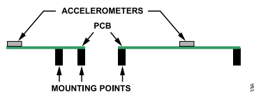
Figure 35. Incorrectly Placed Accelerometers
