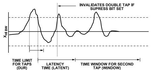
Figure 37. Double Tap Event Invalid Due to High g Event When the Suppress Bit Is Set
