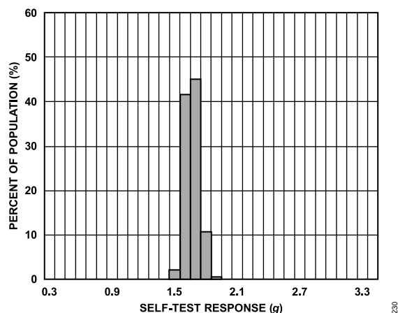
Figure 21. Z-Axis Self-Test Response at 25°C, V_S = 2.5\text{ V}
