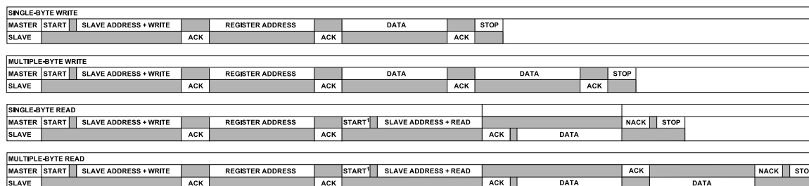
Figure 31. I 2 C Device Addressing
