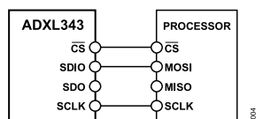
Figure 24. 3-Wire SPI Connection Diagram
