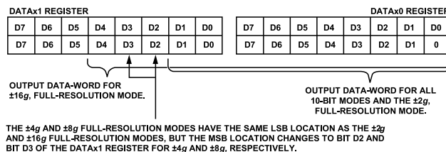
Figure 39. Data Formatting of Full-Resolution and \pm 2 g, 10-Bit Modes of Operation When Output Data Is Right Justified
