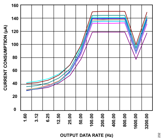
Figure 22. Current Consumption vs. Output Data Rate at 25°C—10 Parts, V_S = 2.5\text{ V}
