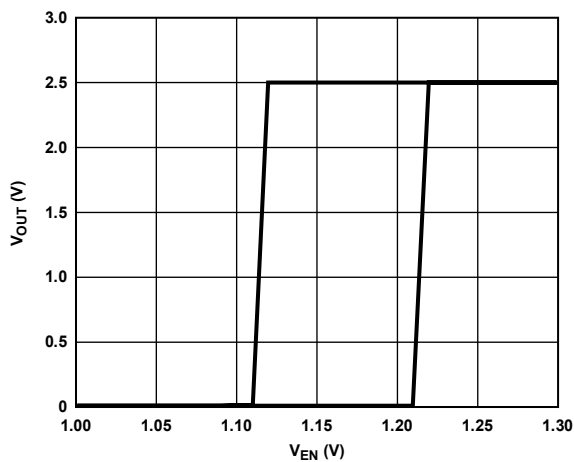
Figure 58. Typical VOUT Response to EN Pin Operation
