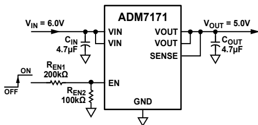
Figure 59. Typical EN Pin Voltage Divider
