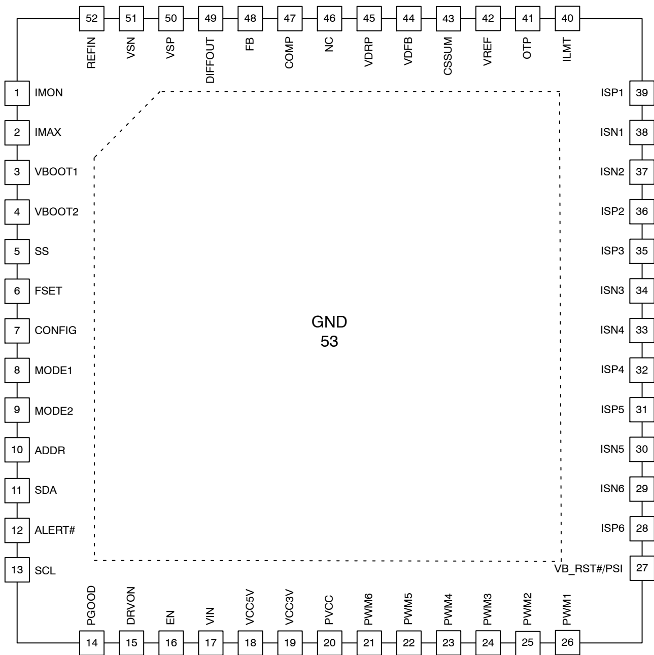
Figure 1. Pin Configuration
