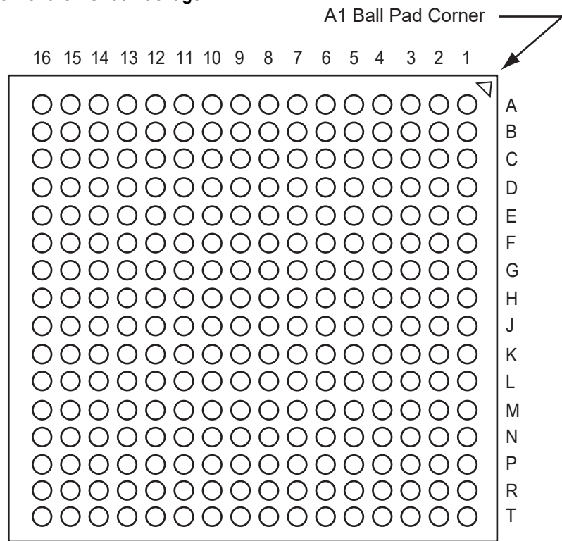
Figure 64 • Top-view of the FG256 Package
