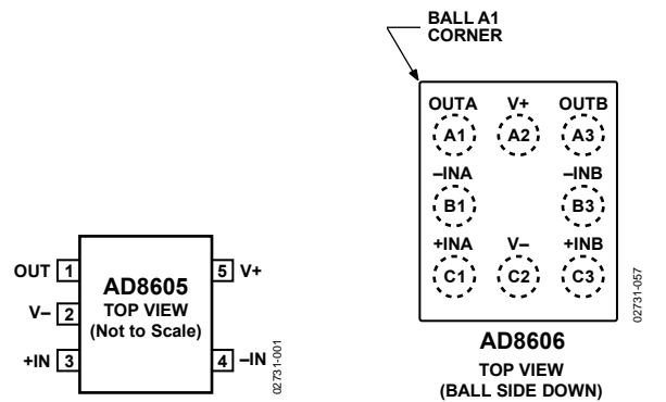
Figure 1. 5-Lead SOT-23 (RJ Suffix)
