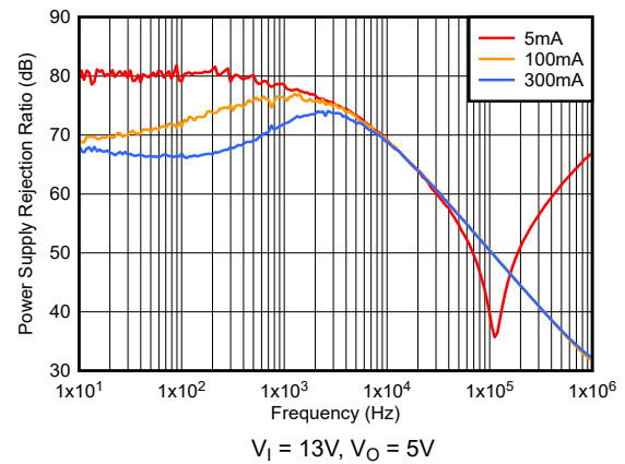
Figure 5-10. PSRR vs Frequency and I_O (New Chip)
