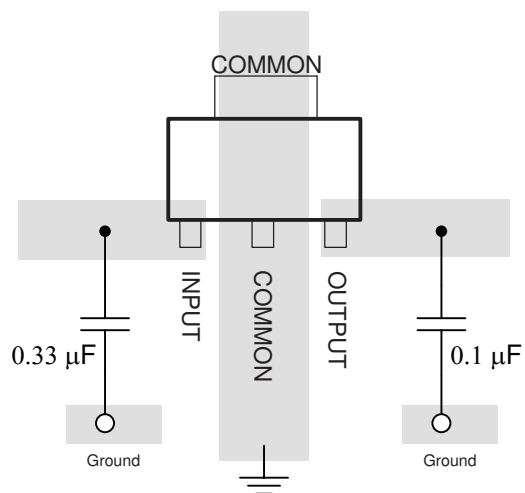
Figure 7-12. Layout Diagram
