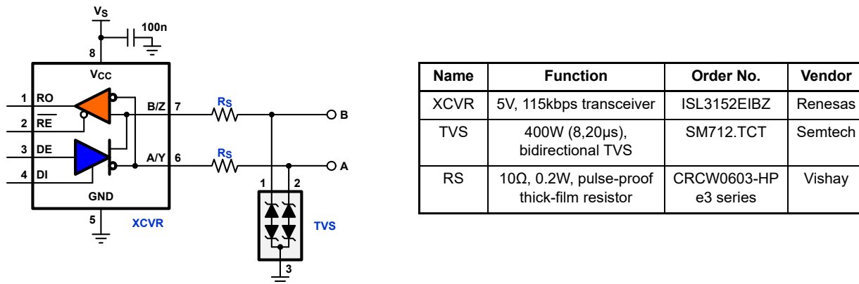
Figure 43. IEC61000-4-5 Level 2 (1kV) Surge Protection and Associated Bill of Materials
