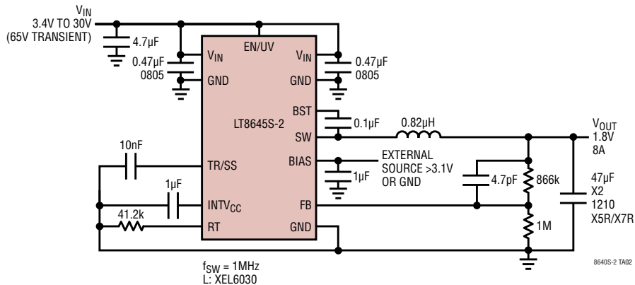
1.8V, 8A Step-Down Converter
