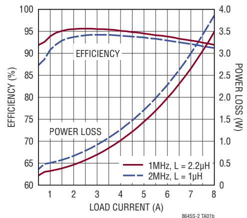
12VIN to 5VOUT Efficiency
