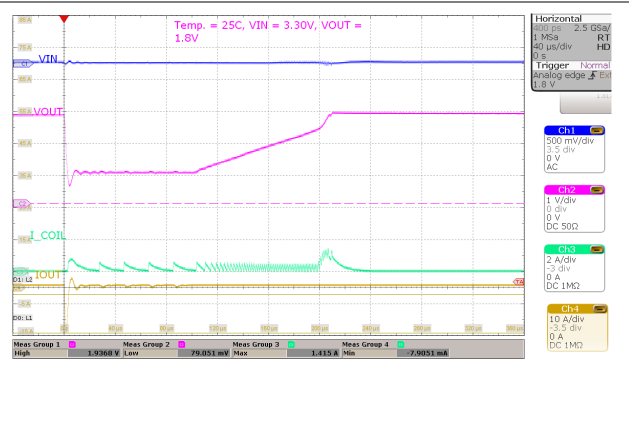
Figure 8-39. Short Circuit Behavior
