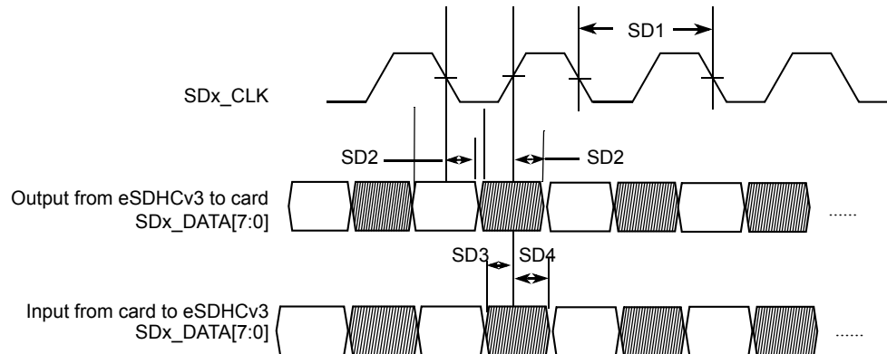
Figure 38. eMMC4.4/4.41 Timing
