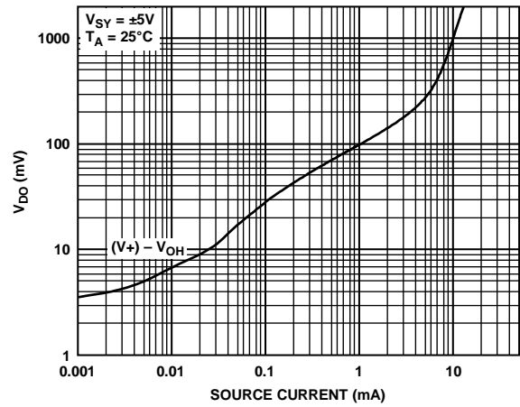
Figure 52. Dropout Voltage ( V_{D0} ) vs. Source Current
