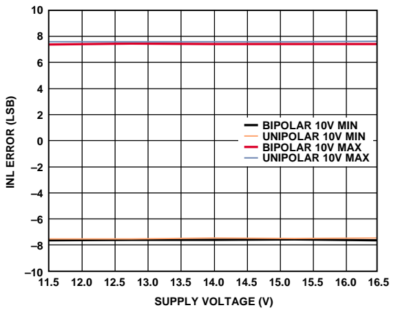
Figure 14. AD5752R Integral Nonlinearity Error vs. Supply Voltage
