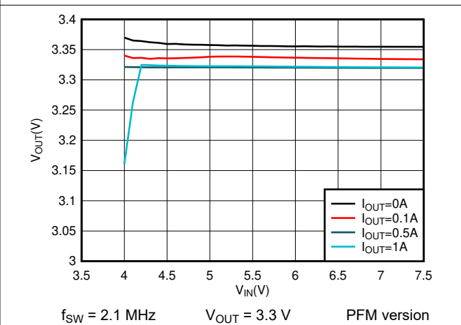
Figure 7-6. 3.3-V Dropout
