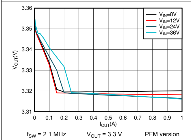
Figure 7-3. 3.3-V Load Regulation
