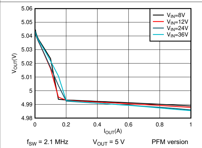
Figure 7-4. 5-V Load Regulation
