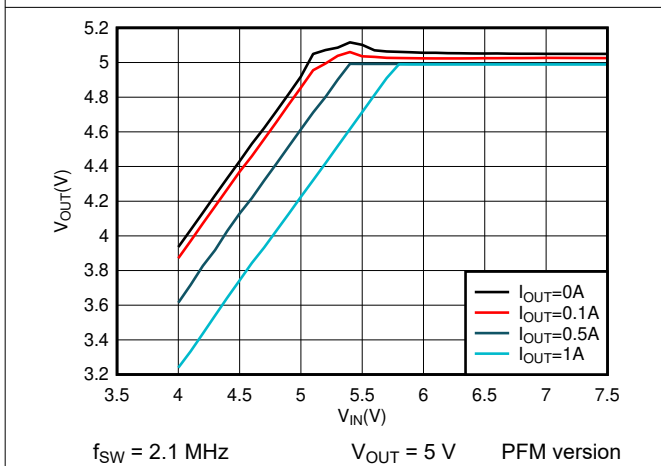
Figure 7-5. 5-V Dropout
