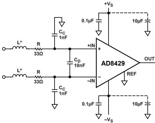
*CHIP FERRITE BEAD. Figure 53. RFI Suppression
