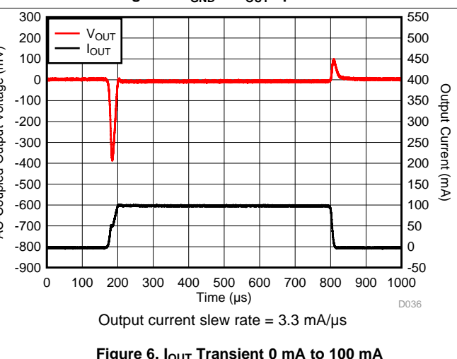
Figure 6. I_{OUT} Transient 0 mA to 100 mA
