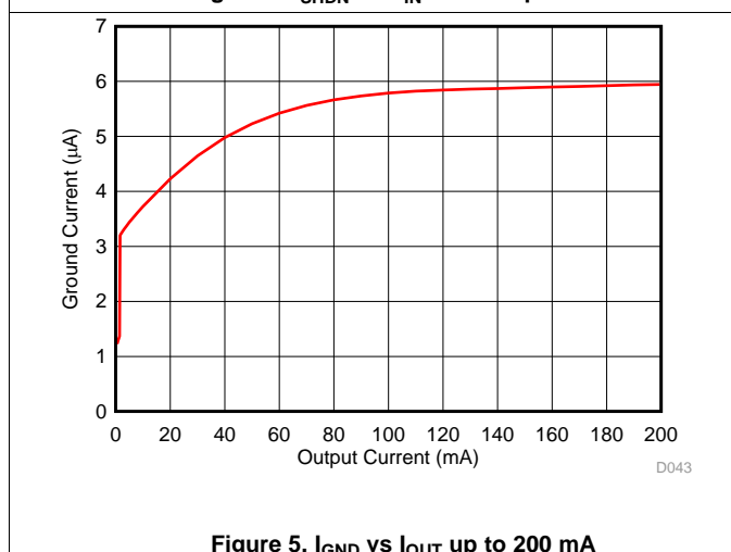
Figure 5. I_{GND} vs I_{OUT} up to 200 mA
