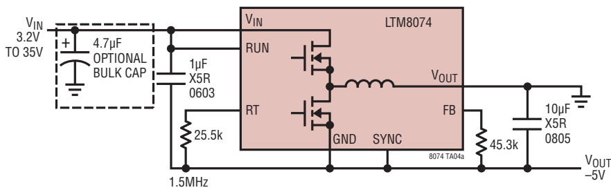
-5V OUT from 3.2V IN to 35V IN Positive to Negative Converter
