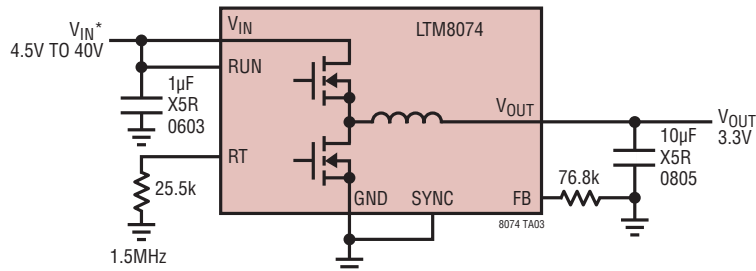
3.3V OUT from 4.5V IN to 40V IN Step-Down Converter
