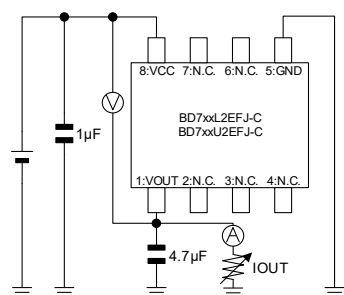
Measurement setup for Figure 9, 19
