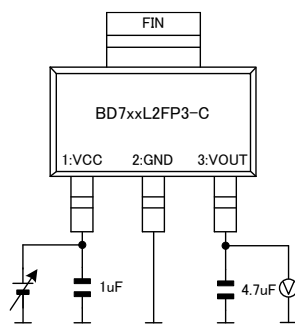
Measurement setup for Figure 6, 7, 12, 13, 16, 17, 22, 23
