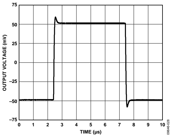
Figure 35. Small Signal Transient Response, V_{SY} = \pm 5 V , A_v = 1 , R_L = 2 k\Omega , C_L = 100 pF
