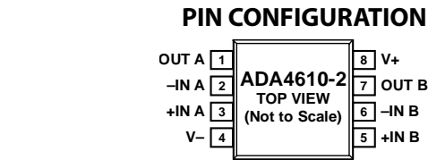
Figure 1. ADA4610-2 8-Lead SOIC (R Suffix); for Additional Packages and Models, See the Pin Configurations and Function Descriptions Section
