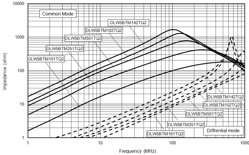
DLW5BT_TQ series
