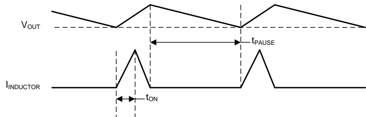
Figure 4. Power Save Mode Waveform Diagram
