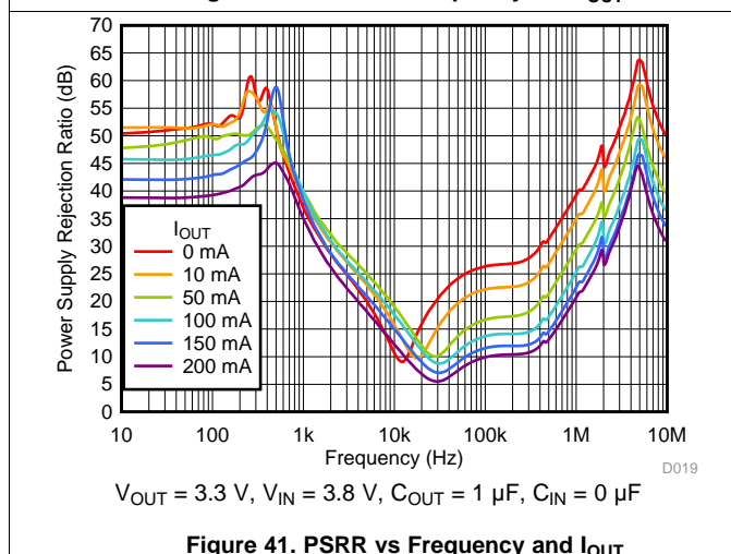
Figure 41. PSRR vs Frequency and I_{OUT}
