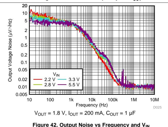
Figure 42. Output Noise vs Frequency and V_{IN}
