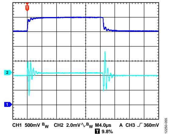
Figure 54. Line Transient Response, 2.5 V to 3 V, I_{LOAD} = 2\text{ A} , Adjustable Version, V_{OUT} = 1.2\text{ V} , CH1 = V_{IN} , CH2 = V_{OUT}
