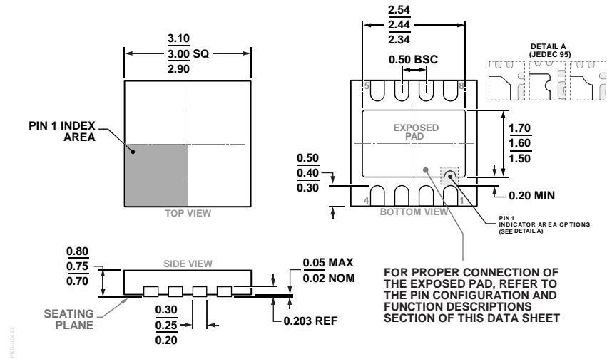
Figure 71. 8-Lead Lead Frame Chip Scale Package [LFCSP] 3 mm x 3 mm Body and 0.75 mm Package Height (CP-8-21) Dimensions shown in millimeters
