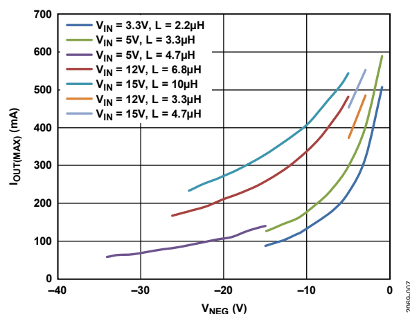
Figure 8. Inverting Regulator Maximum Output Current, f_{SW} = 2.4 MHz, T_A = 25^\circ C , Based on Target of 70% I_{LIM(INVERTER)}
