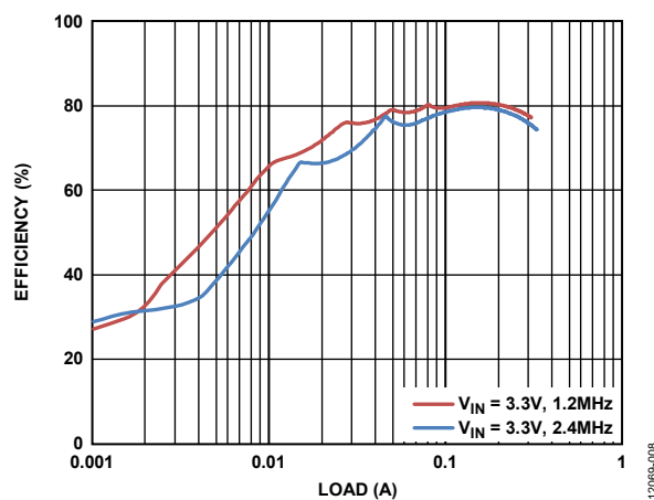
Figure 9. Inverting Regulator Efficiency vs. Current Load, V_{IN} = 3.3 V, V_{NEG} = -5 V, T_A = 25^\circ C
