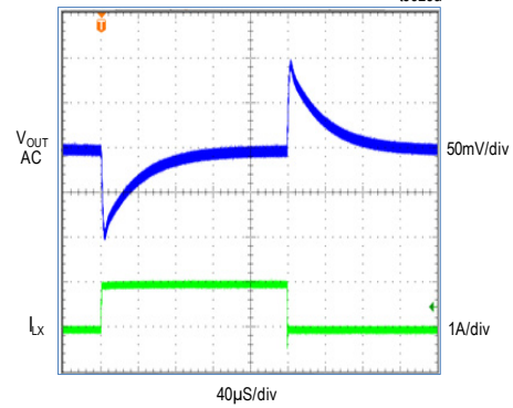
MAX17503S, 3.3V OUTPUT, PWM MODE, FIGURE 4d CIRCUIT (LOAD CURRENT STEPPED FROM NO LOAD TO 1A)
