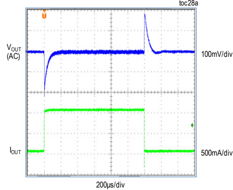
MAX17503S, 5V OUTPUT, DCM MODE (LOAD CURRENT STEPPED FROM 50mA TO 1A) FIGURE 4c CIRCUIT
