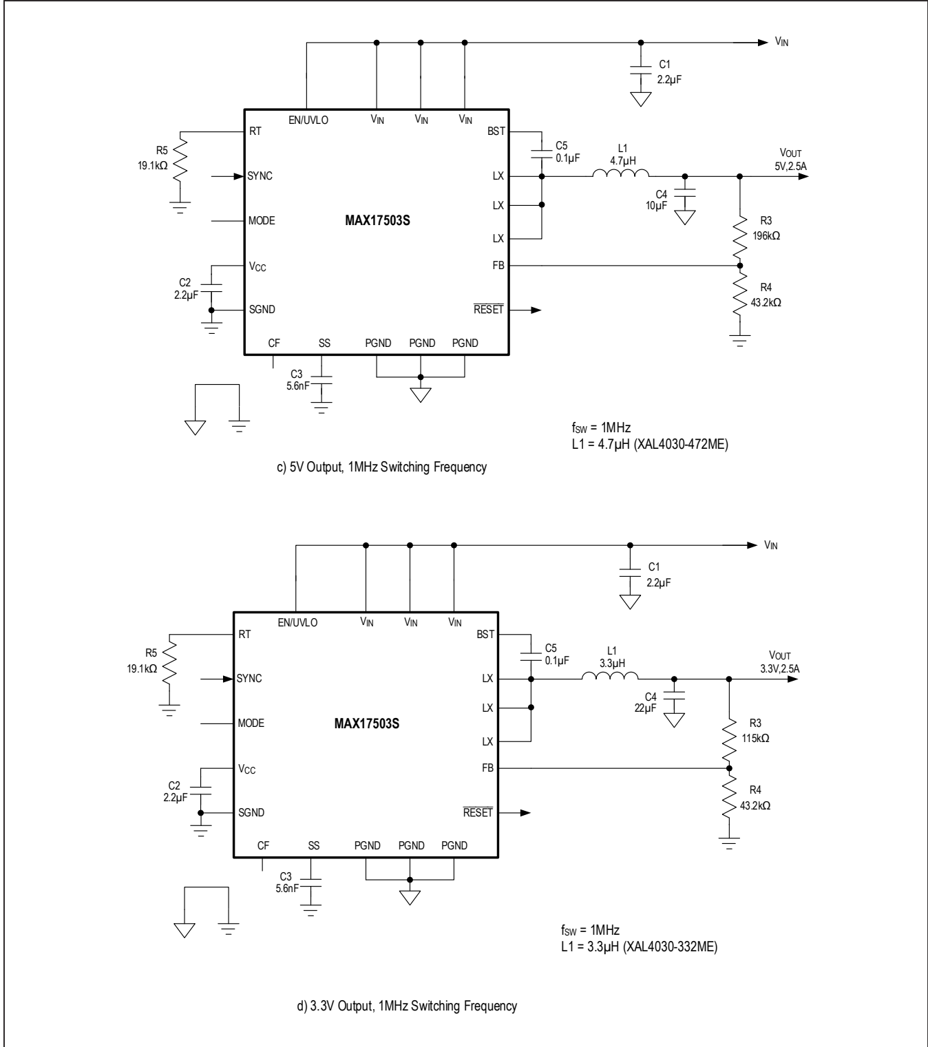
Figure 4. MAX17503/MAX17503S Typical Application Circuits (continued)
