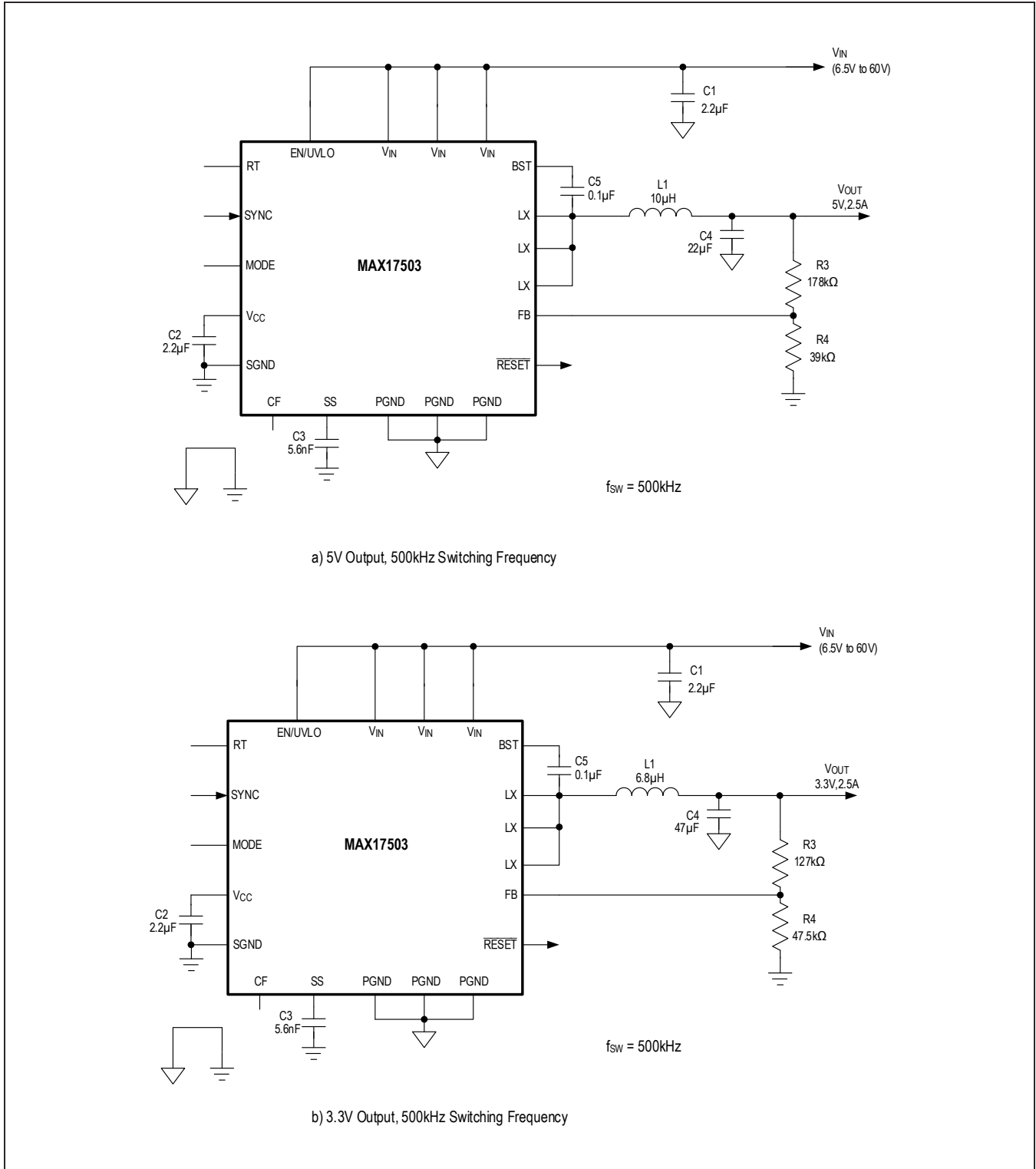
Figure 4. MAX17503/MAX17503S Typical Application Circuits
