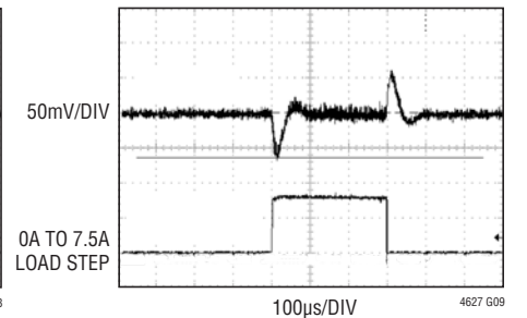
1.8V Transient Response
