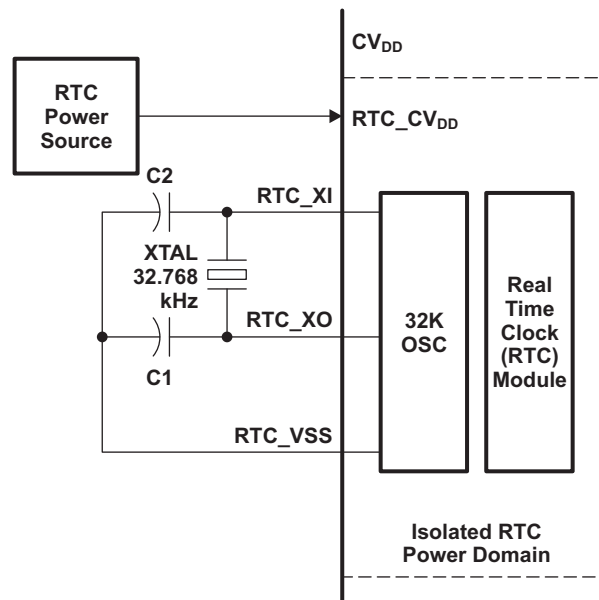
Figure 5-83. Clock Source
