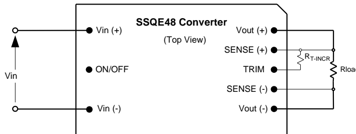
Figure C. Configuration for increasing output voltage.
