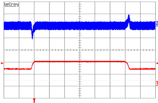
Figure 8. Output voltage response to load current step-change (6.5 A–9.75 A–6.5 A) at V_{in} = 48\text{ V} . Top trace: output voltage (100 mV/div.). Bottom trace: load current (5 A/div.). Current slew rate: 0.1A/ \mu\text{s} . C_o = 1\mu\text{F} ceramic + 10 \mu\text{F} tantalum. Time scale: 0.2 ms/div.
