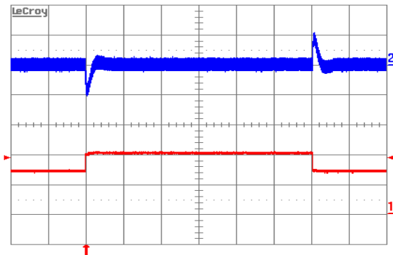
Figure 9. Output voltage response to load current step-change (6.5 A–9.75 A–6.5 A) at V_{in} = 48\text{ V} . Top trace: output voltage (100 mV/div.). Bottom trace: load current (5A/div.). Current slew rate: 5 A/ \mu\text{s} . C_o = 470\mu\text{F} POS + 1 \mu\text{F} ceramic. Time scale: 0.2 ms/div.
