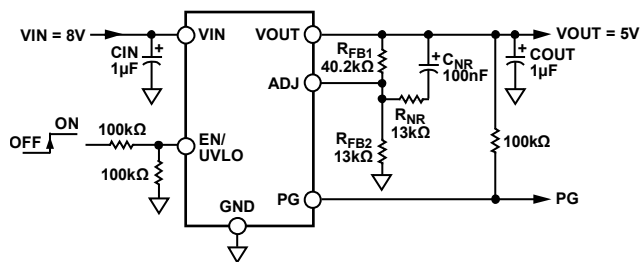
Figure 70. Noise Reduction Modification to Adjustable LDO
