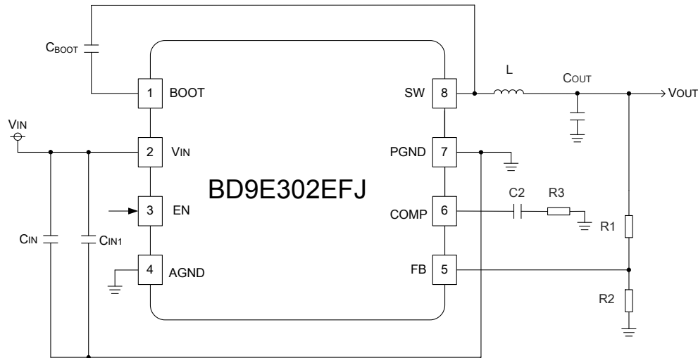
Figure 56. Application Circuit 3
