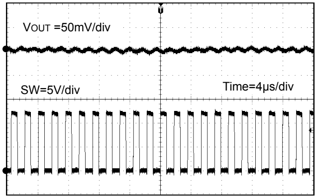
Figure 34. SW Waveform (②PWM control) ( V_{in} = 12V , V_{out} = 5.0V , I_{out} = 3A )
