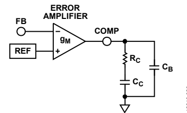
Figure 26. Compensation Components
