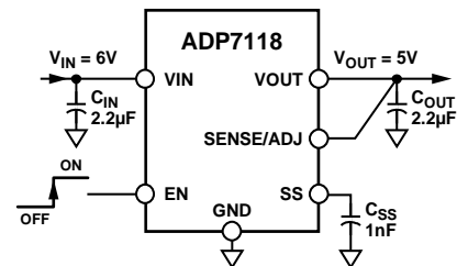
Figure 1. ADP7118 with Fixed Output Voltage, 5 V
