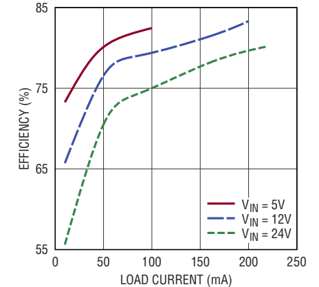
Efficiency vs Load Current, V_{OUT} = 15\text{V}
