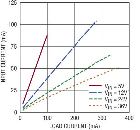
Input Current vs Load Current V_{OUT} = 3.3\text{V}
