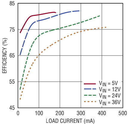
Efficiency vs Load Current, V_{OUT} = 8\text{V}
