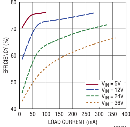
Efficiency vs Load Current, V_{OUT} = 3.3\text{V}
