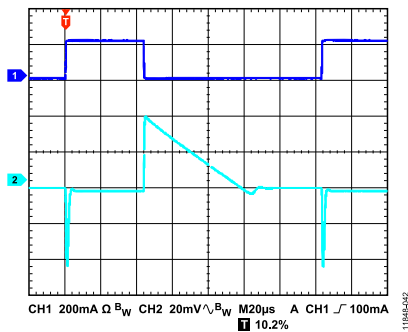
Figure 44. Output Transient Response, V_{OUT} = 5 V, C_{OUT} = 2.2 μF, CH1 Load Current, CH2 V_{OUT}
