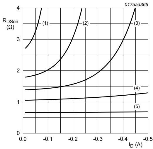
Fig. 8. Drain-source on-state resistance as a function of drain current; typical values (1) V_{GS} = -1.5\text{ V} (2) V_{GS} = -1.8\text{ V} (3) V_{GS} = -2.0\text{ V} (4) V_{GS} = -2.5\text{ V} (5) V_{GS} = -4.5\text{ V}
