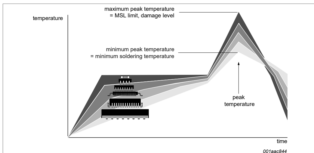
Figure 22. Temperature profiles for large and small components
