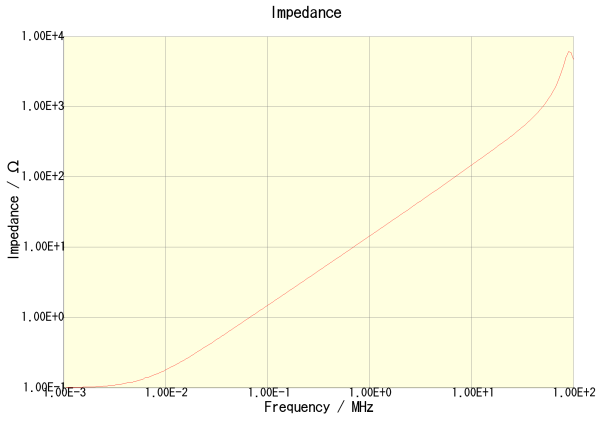
CLF12555T-2R2N-CA
