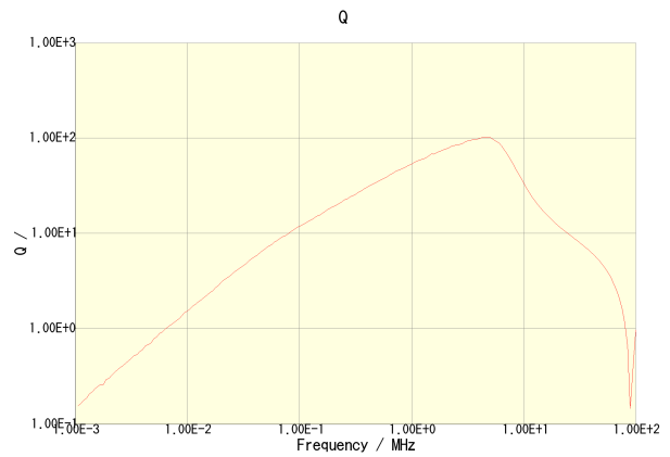
CLF12555T-2R2N-CA
