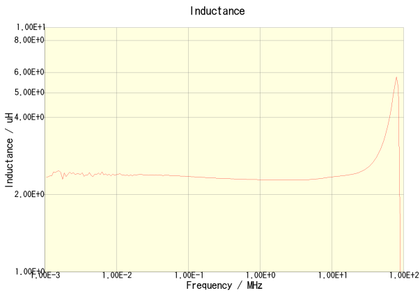
CLF12555T-2R2N-CA
