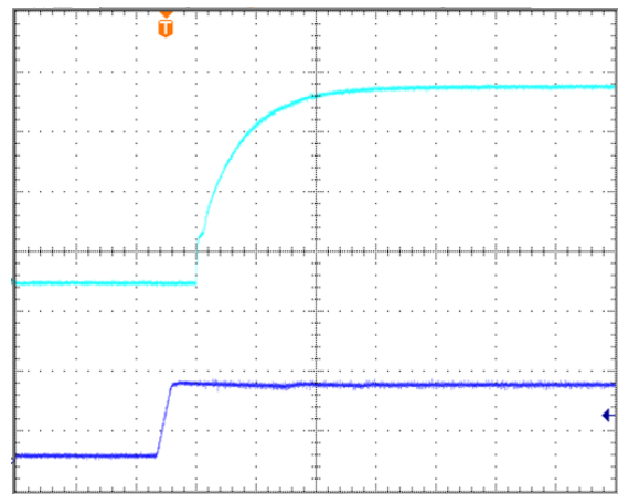
Turn-on transient at full load current (10ms/div). Top Trace: Vout; 1V/div; Bottom Trace: input voltage: 20V/div.
