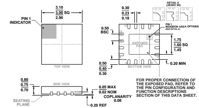
COMPLIANT TO JEDEC STANDARDS MO-220-WEED-6. Figure 27. 16-Lead Lead Frame Chip Scale Package [LFCSP] 3 mm × 3 mm Body and 0.75 mm Package Height (CP-16-22) Dimensions shown in millimeters
