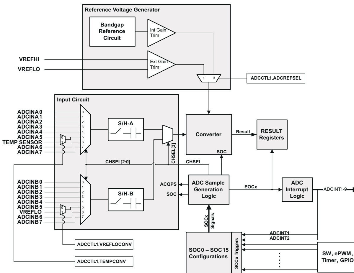
Figure 8-1. ADC Block Diagram
