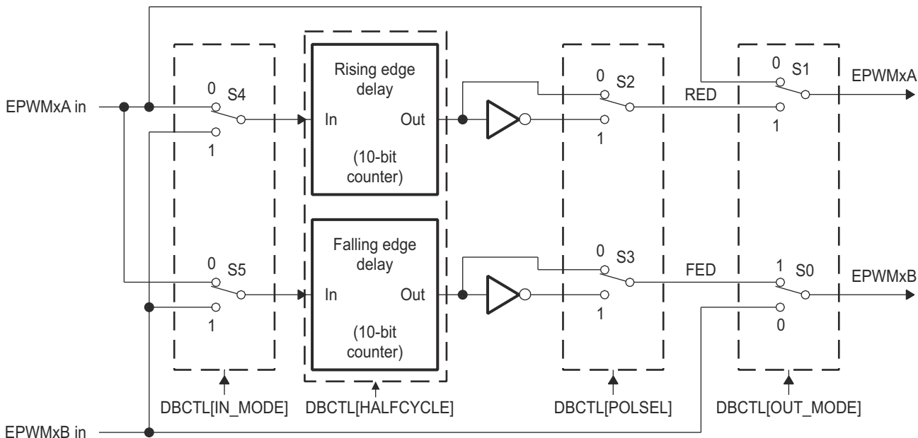
Figure 3-29. Configuration Options for the Dead-Band Submodule
