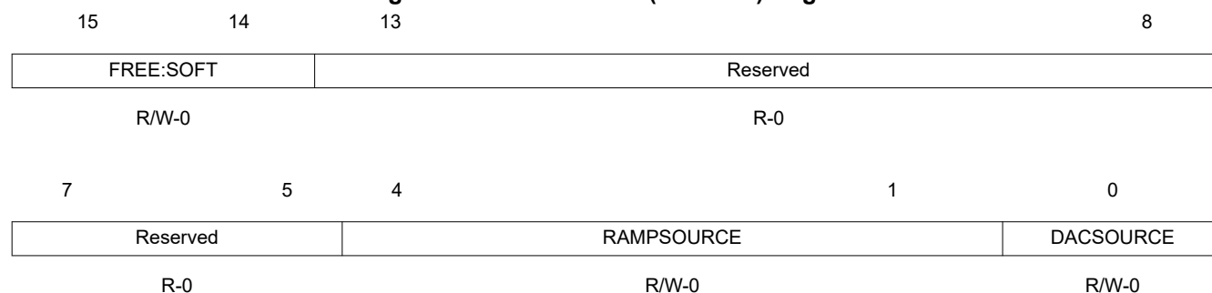
Figure 9-7. DAC Control (DACCTL) Register
