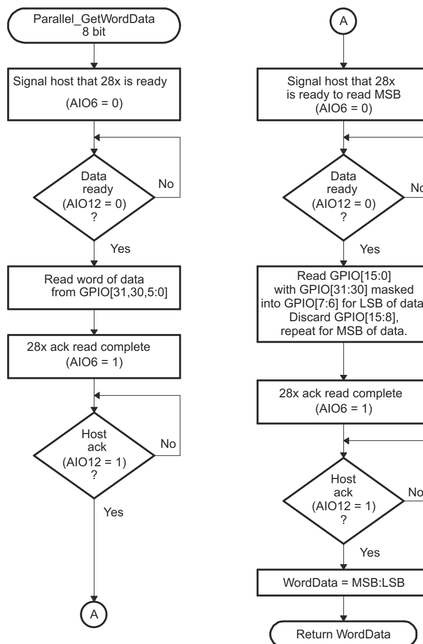
Figure 2-19. 8-Bit Parallel GetWord Function
