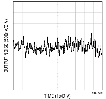
2.5V Low Frequency 0.1Hz to 10Hz Noise
