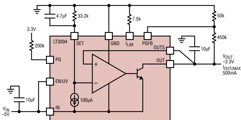
PIN NOT USED IN THIS CIRCUIT: VIOC
