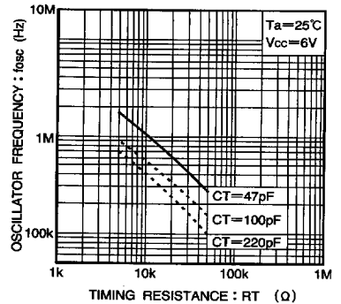
Fig.3 Triangle oscillation frequency vs. timing resistance
