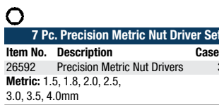
7 Pc. Precision Metric Nut Driver Set Item No. Description Case Pack 26592 Precision Metric Nut Drivers 3 Metric: 1.5, 1.8, 2.0, 2.5, 3.0, 3.5, 4.0mm
