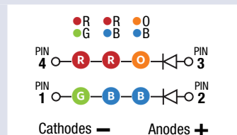
Schematic
