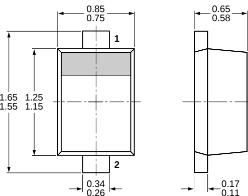
Dimensions in mm 02-12-13
