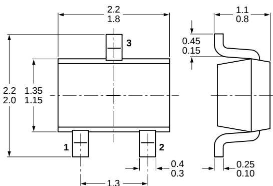
Dimensions in mm 04-11-04
