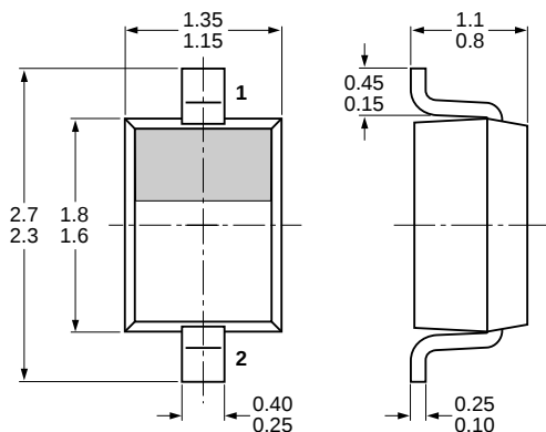
Dimensions in mm 03-12-17
