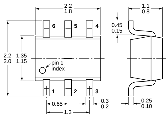
Dimensions in mm 06-03-16
