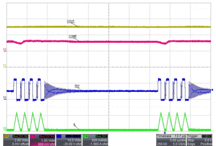
Figure 5: PFM Mode at Light Load (5 mA) V_{IN} = 12V, V_{OUT} = 5.0V
