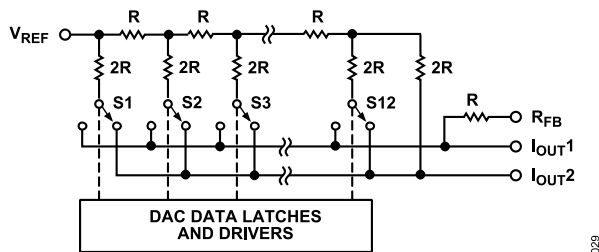
Figure 37. Simplified Ladder
