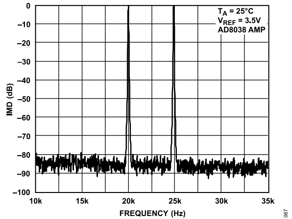
Figure 34. Narrow-Band IMD, f_{OUT} = 20 kHz and 25 kHz, Clock = 1 MHz
