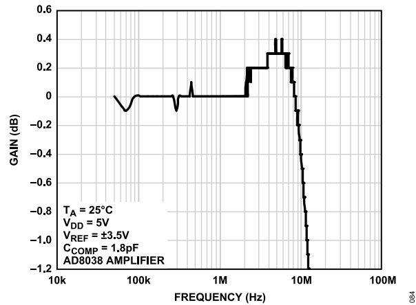
Figure 23. Reference Multiplying Bandwidth vs. Frequency—All 1s Loaded
