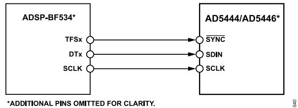
Figure 48. ADSP-BF534 to AD5444/AD5446 Interface
