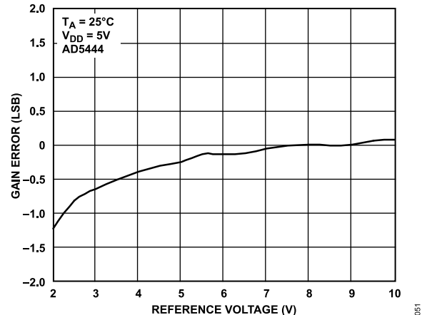
Figure 16. Gain Error vs. Reference Voltage
