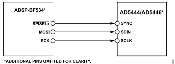
Figure 47. ADSP-BF534 to AD5444/AD5446 Interface
