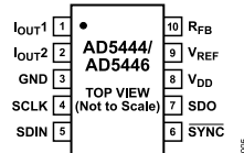
Figure 5. Pin Configuration
