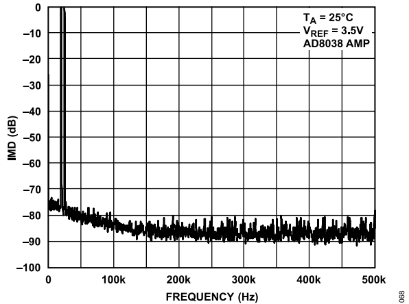
Figure 35. Wideband IMD, f_{OUT} = 20 kHz and 25 kHz, Clock = 1 MHz
