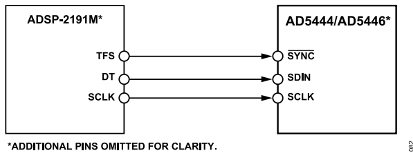
Figure 46. ADSP-2191M to AD5444/AD5446 Interface
