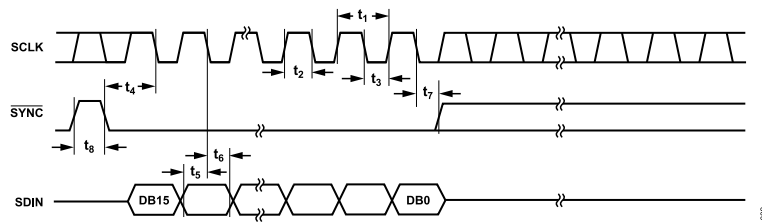
Figure 2. Standalone Timing Diagram
