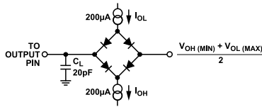
Figure 4. Load Circuit for SDO Timing Specifications
