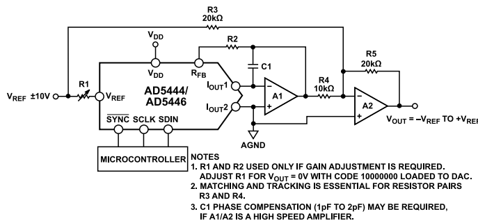
Figure 39. Bipolar Operation (4-Quadrant Multiplication)
