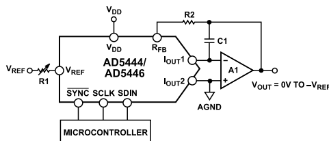
Figure 38. Unipolar Operation
