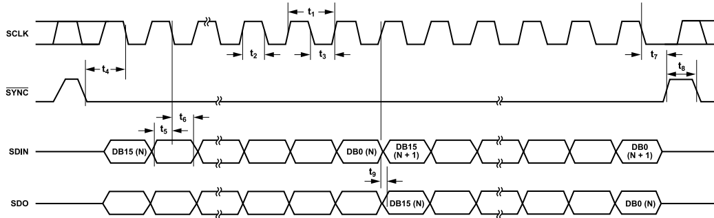
Figure 2. Standalone Timing Diagram
