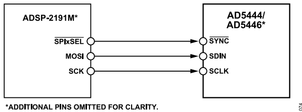
Figure 45. ADSP-2191M SPI to AD5444/AD5446 Interface
