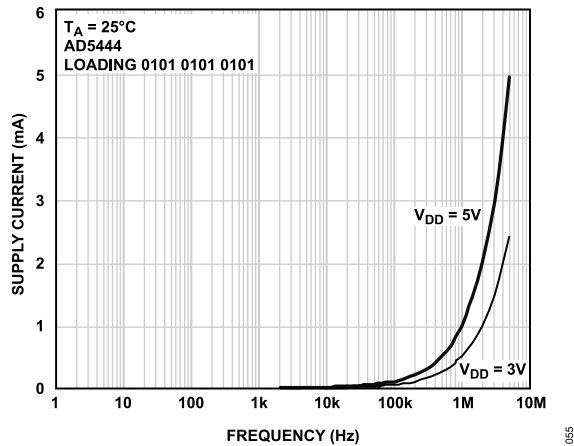
Figure 20. Supply Current vs. Update Rate
